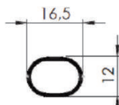
TUBO OBLONGO 16,5 X 12 X 1,2MM
