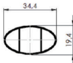
TUBO ELIPTICO 35 X 20 X 1,3MM C/ ALMA
