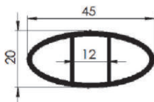
TUBO ELIPTICO 45 X 20 X 1,6MM C/ ALMA
