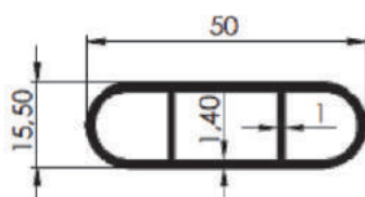
TRAVESSA 50 x 15 x 1,4 X 1,0
